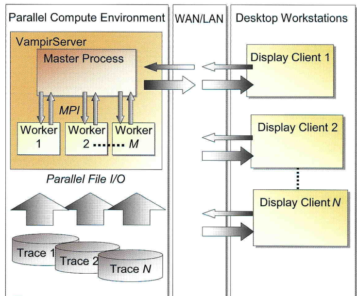
The distributed analysis architecture of VampirServer
